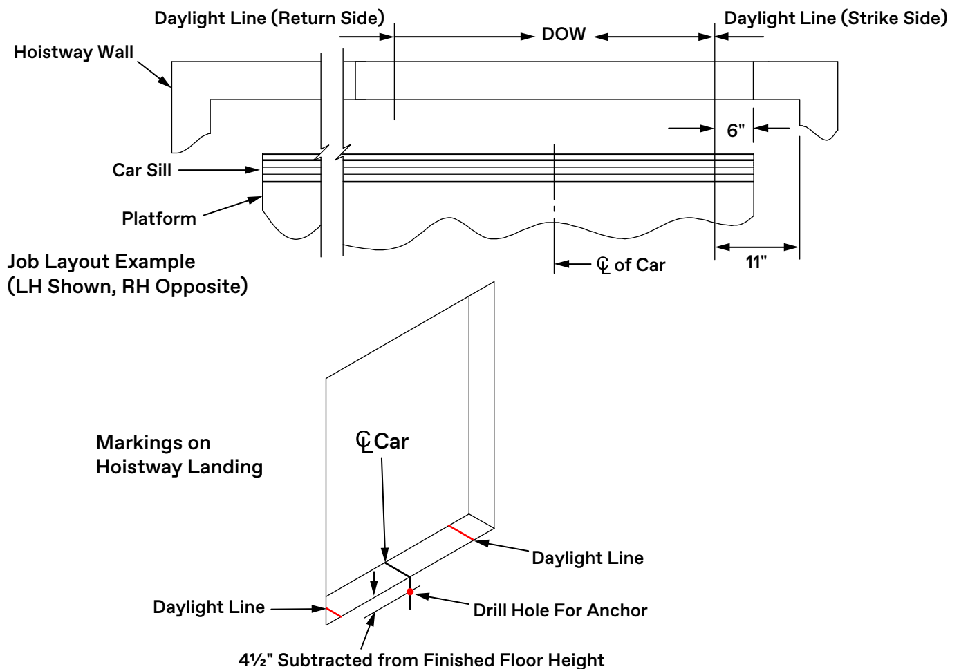
Figure 18 - Sill Installation (1 of 2)
