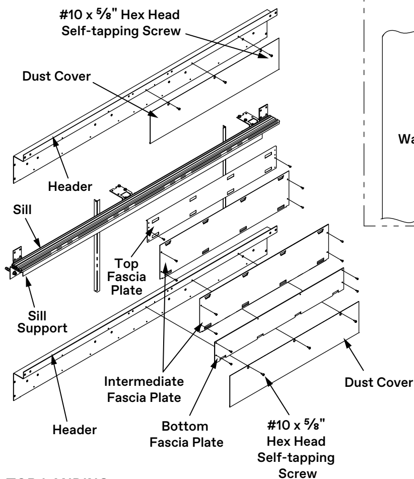
TOP LANDING
