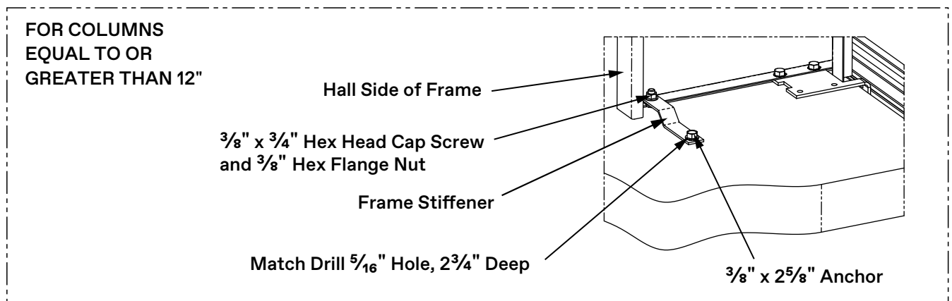
Figure 7 - Install Entrance Frame
