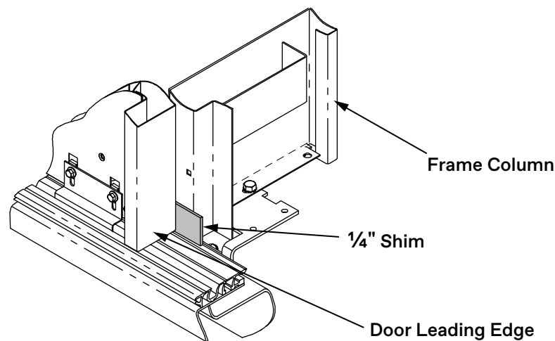
Figure 12 - Adjust Door Gibs
