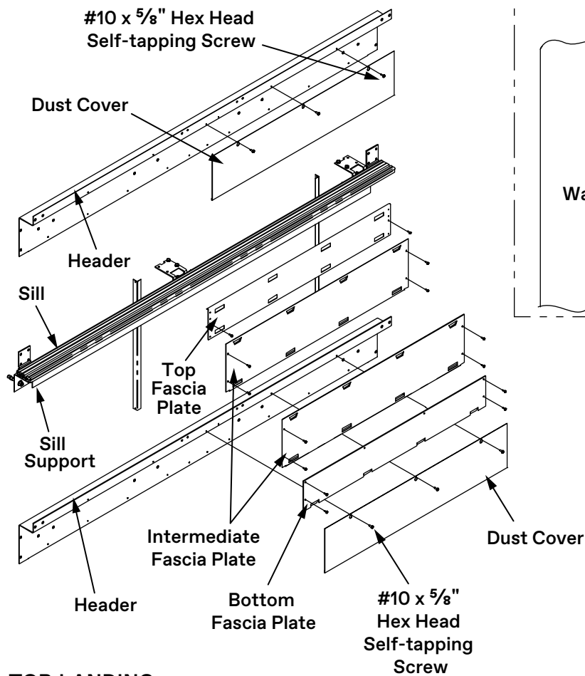
TOP LANDING
