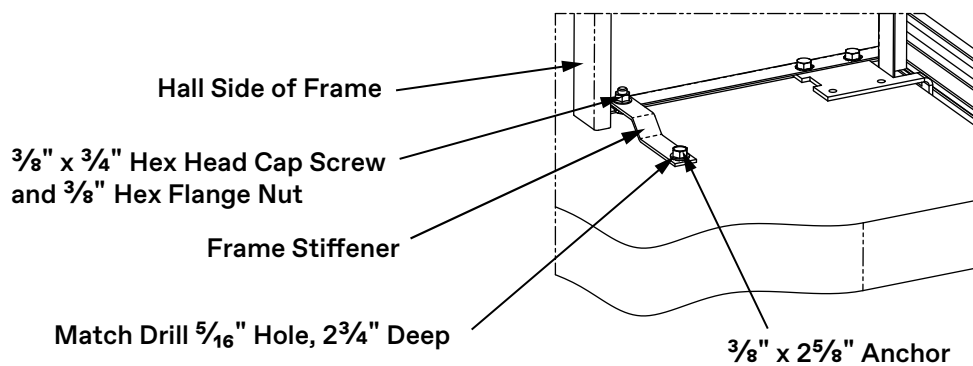
Figure 42 - Install Entrance Frame
